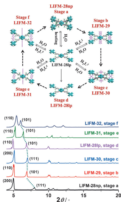
Figure 2. Top: Stepwise installation/uninstallation from \text{H}_2\text{L}^2 to \text{H}_2\text{L}^5 mediated by reversible PVSIs processes with LIFM-28lp crystals to achieve different stages of breathing behaviors in a continuous way. Bottom: Elastic deformation in six stages reflected by specific PXRD peaks shift.
